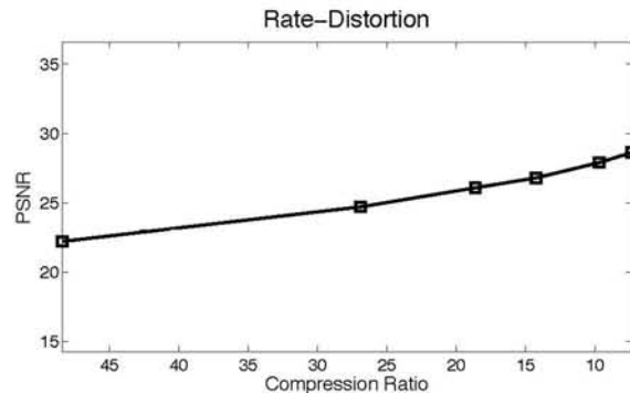
Fig. 6. Rate-Distortion curve for the video sequence. The PSNR for each bit-rate is the average of all 100 frames in the sequence.
